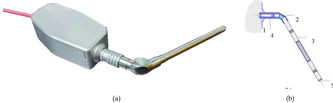
Fig. 3. Optical setup of bayonet-shaped probe for CP OCT: (a) external view; (b) schematic and. 1 – telecentric scanning lens group, 2 – probe folding, 3 – replaceable sterilizable optical beam translator, 4 – standard LEMO's® coupling, 5 – main optical axis
